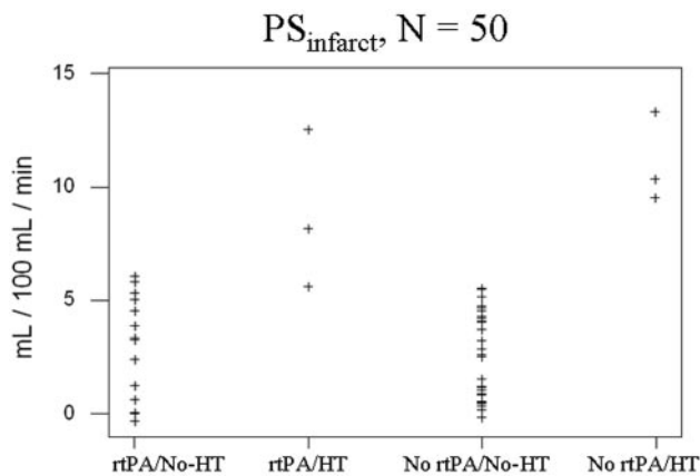
Fig 4. Scatterplot of the 50 PS infarct values, categorized by whether emergent rtPA was given and whether subsequent HT occurred. Note the separation of PS HT values (second and fourth columns) from those of PS No-HT (first and third columns).
