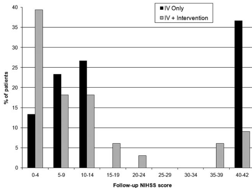
Fig 2. Graph shows the distribution of NIHSS scores at follow-up for patients in each group, displayed in a relative-frequency histogram. Black bars indicate patients who received IV rPA but no endovascular intervention. Gray bars indicate patients who received IV rPA followed by endovascular intervention. NIHSS scores at follow-up were significantly better in patients who received IV rPA plus endovascular intervention ( P = .037 ).
