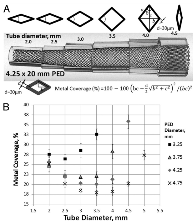
FIG 1. A, Representative image of a 4.25 × 20 mm Pipeline device inserted into plastic tubes of 0.5-mm incremental diameters. Variation in the degree of metal coverage is apparent. The configuration of cells is schematically depicted above the construct. Metal coverage can be calculated directly on the basis of measurements of the long and short diagonals of the rhombus and the diameter of each strand (30- \mu\text{m} ), according to the formula above. Minimum coverage is seen when \theta = 90^\circ , corresponding to a square cell configuration. B, Scatterplot of tube diameter versus metal coverage for various device and “artery” combinations. All functions have a parabolic configuration. Note that absolute coverage values are higher for smaller diameter devices at each given tube diameter. The overall single-device coverage is, therefore, likely to be somewhat smaller for appropriately sized devices deployed in larger vessels.
