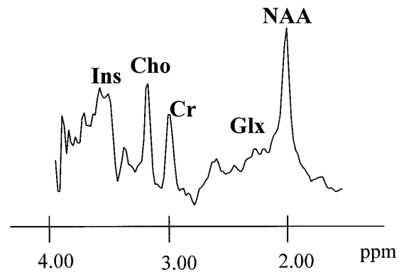
Fig 4. A proton MR spectrum (25/2000) obtained from the white matter of a 34-year-old patient with MS. A 15 \times 15 \times 15 -mm 3 (3.4-mL) volume of interest was located in the left temporooccipital white matter of brain (see Fig 6). The high Cho peak is characteristic of the spectra from this group of patients. (See legend to Figure 1 for definition of abbreviations.)
