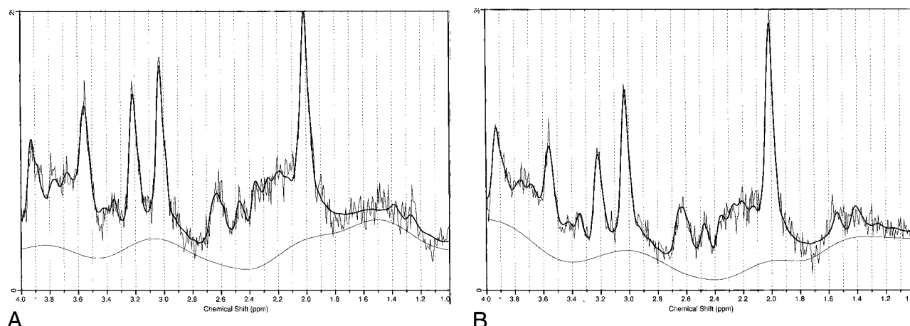
FIG 2. Proton spectra from same subject and voxel locations as shown in Figure 1. The dark line represents the LCMoDel fit of the spectrum. The assignments of the principal peaks (in ppm) in the in vivo spectrum are as follows: NA = NAA (2.01) + NAAG (2.05), Cr (3.03), Ins (3.56). The complex multiplets of Glu and Gln, whose sum is Glx, are located at approximately 2.1 to 2.5 ppm and 3.7 to 3.8 ppm (see [41]).
