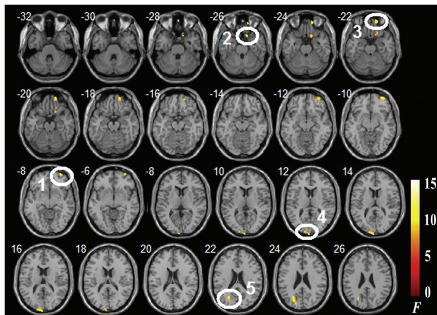
FIG 1. Regions with differences in regional homogeneity among the CID-NI, CID-MCI, and NC groups (voxels at least 60, P < .001 ). 1) Right inferior frontal gyrus. 2) Right superior frontal gyrus. 3) Right orbital middle frontal gyrus. 4) Left cuneus. 5) Left superior occipital gyrus.
