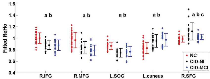
FIG 2. Plot of the regional homogeneity index among the CID-NI, CID-MCI, and NC groups in the identified brain regions (voxels at least 60, P < .001 ). a, The ReHo index is significantly different between the NC and CID-MCI groups. b, The ReHo index is significantly different between the NC and CID-NI groups. c, The ReHo index is significantly different between the CID-MCI and CID-NI groups. R indicates right; L, left; IFG, inferior frontal gyrus; MFG, middle frontal gyrus; SOG, superior occipital gyrus.
