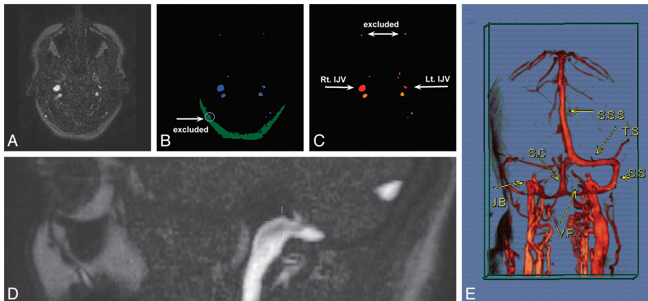
FIG 1. Example of vein detection and mapping algorithms in 1 participant. The original phase-contrast MR image at the level of the JF (A) was initially processed by the vein detection algorithm according to intensity levels (B). Blue represents pixels that surpassed a high-intensity threshold. Yellow stands for pixels between medium and high-intensity thresholds attached to high-intensity objects. The vein cross-sectional area was determined by the sum of both blue and yellow areas. Green corresponds to low-intensity subcutaneous fat tissue. Detected veins in this tissue drain the scalp and therefore were excluded (white arrow). The resulting image was further processed by the mapping algorithm according to size and location (C). The 2 most anterior veins were identified as facial veins and thus were excluded. Vessels anterior to the jugular veins (red) were considered to be the pterygopalatine plexus (purple). Vessels posterior to the jugular veins were regarded as the vertebral plexus (orange). The level of image acquisition (JF) is also presented (D). E, Illustrative contrast-enhanced MR venography with 3D reconstruction demonstrates venous drainage of the brain: S.S.S., superior sagittal sinus; T.S., transverse sinus; S.S., sigmoid sinus; S.C., sinus cerebella; J.B., jugular bulb; V.P., vertebral plexus.
