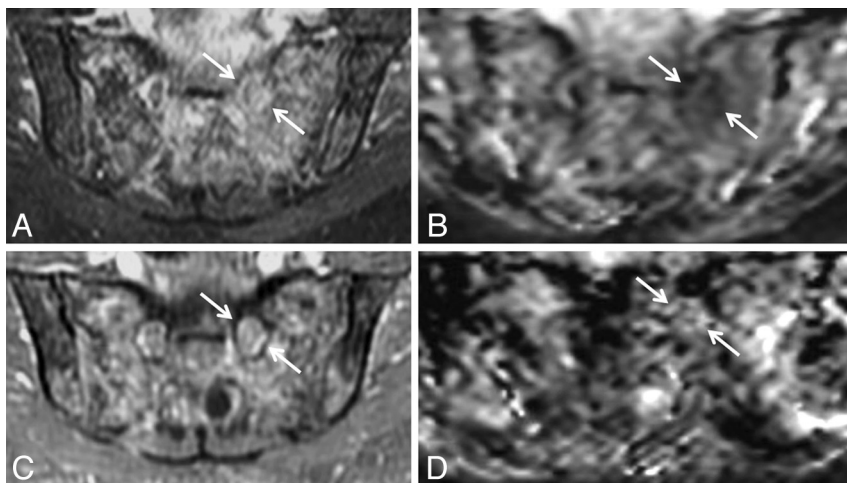
FIG 9. Marked increase in diffusivity following radiation therapy for metastatic breast cancer in a 47-year-old woman with pain in the left L4 through S2 distribution. Axial fat-saturated postgadolinium T1 and ADC before (A and B) and 4 months following completion of radiation therapy (C and D). Initial images (A and B) demonstrate metastatic disease throughout the sacrum and infiltrating the left S1 nerve (arrows). B, Before radiation, ADC within the diseased left S1 nerve was 0.78 \pm 0.15 \times 10^{-3} \text{ mm}^2/\text{s} . D, Four months later, following completion of radiation therapy, ADC within the nerve had markedly increased to 1.39 \pm 0.23 \times 10^{-3} \text{ mm}^2/\text{s} .
