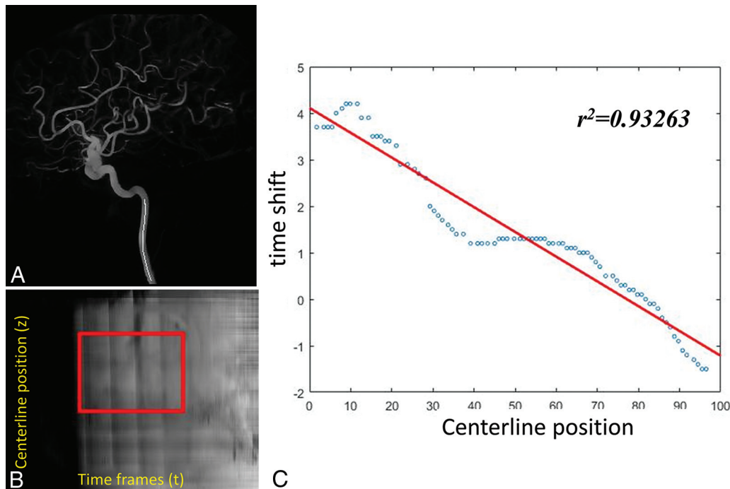
FIG 3. A representative ICA study. A , The centerline positions of the ICA. B , The contrast waveform map of the voxels along the centerline. The highlighted area is the optimized waveform region for the flow calculation. C , The time-shift as a function of the centerline position was fit to a linear relation in which the slope is the inverse of the velocity.
