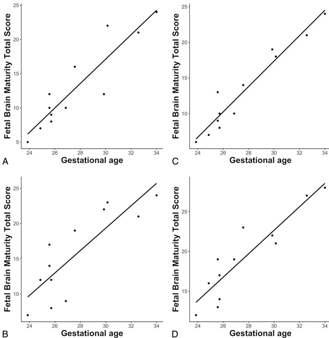
FIG 3. Pearson correlation between GA at MR imaging (x-axis) and the fetal brain maturity total score (y-axis) on the basis of SyMRI-generated (A and B) and conventionally acquired MR imaging data (C and D). Rater 1: A and C; rater 2: B and D.
