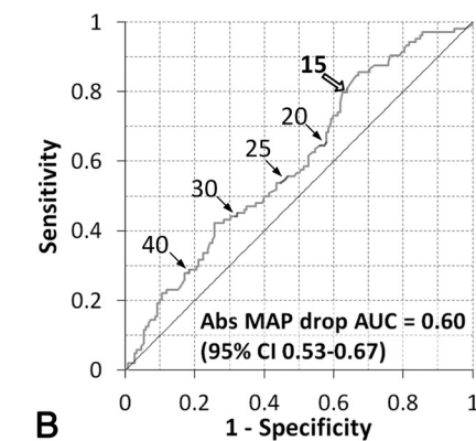
FIG 1. Receiver operating characteristic curves for changes in MAP before modified TICI 2b/3 reperfusion. Curves are shown for the effect of the lowest MAP on 90-day mRS 0–2 (A) and for the relationship between mRS 3–6 and an absolute MAP drop (B) and percentage MAP drop (C). The curves are labeled with pressures (A and B, in millimeters of mercury) and percentages (C). The cutoffs that were independent predictors of outcome in binary regression models are shown with bold type and open block arrows . AUC indicates area under the curve.
