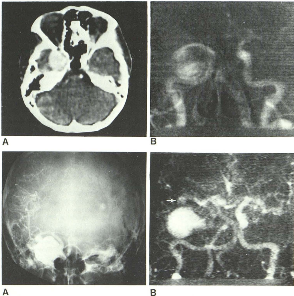
Fig. 2.—Case 2. A, Selective right internal carotid arteriogram. Giant aneurysm of right internal carotid artery and right middle cerebral artery aneurysm. B, Intravenous video arteriogram with 40 ml Renografin-60 (11.6 g I). Giant aneurysm of cavernous segment of right internal carotid artery. Also, aneurysm of right middle cerebral trifurcation (arrow). Overlap of vasculature at base of brain obscures vascular details of circle of Willis.
