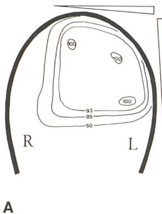
Fig. 10.—Radiation necrosis in 32-year-old man. Left frontal oligodendroglioma treated with 5,000 rad (50 Gy) in 20 fractions over 35 days, as well as radon seed implantation. Severe headache and vomiting 4 years later. Isodose curve (A) and plain (B) and enhanced (C) scans. Extensive area of low density with isodense ring in left frontal region compressing left anterior horn. Marked enhancement. Lesion was excised, revealing radiation necrosis and no tumor.
