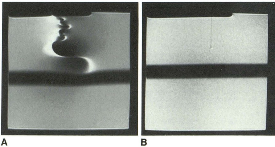
Fig. 1.—A and B, Phantom studies of standard stainless steel (A) and new platinum (B) electrode cannulas (SE/267/30). There is severe geometric and brightness distortion caused by the ferromagnetic properties of the stainless steel but minimal artifact from the platinum.
