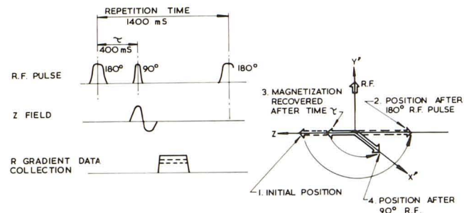
Fig. 3.—Inversion-recovery sequence. One cycle, period 1400 msec, of applied sequence of magnetic fields. Vector diagram illustrates magnitude and direction of magnetization. A 180° RF pulse inverts vector from along +Z direction to -Z direction. After time period \tau of 400 msec, during which some degree of recovery of magnetization along +Z direction occurs, a 90° RF pulse is applied which rotates vector along X' axis. Spatial encoding signal recovery and slice selection then proceed as for saturation-recovery sequence.
