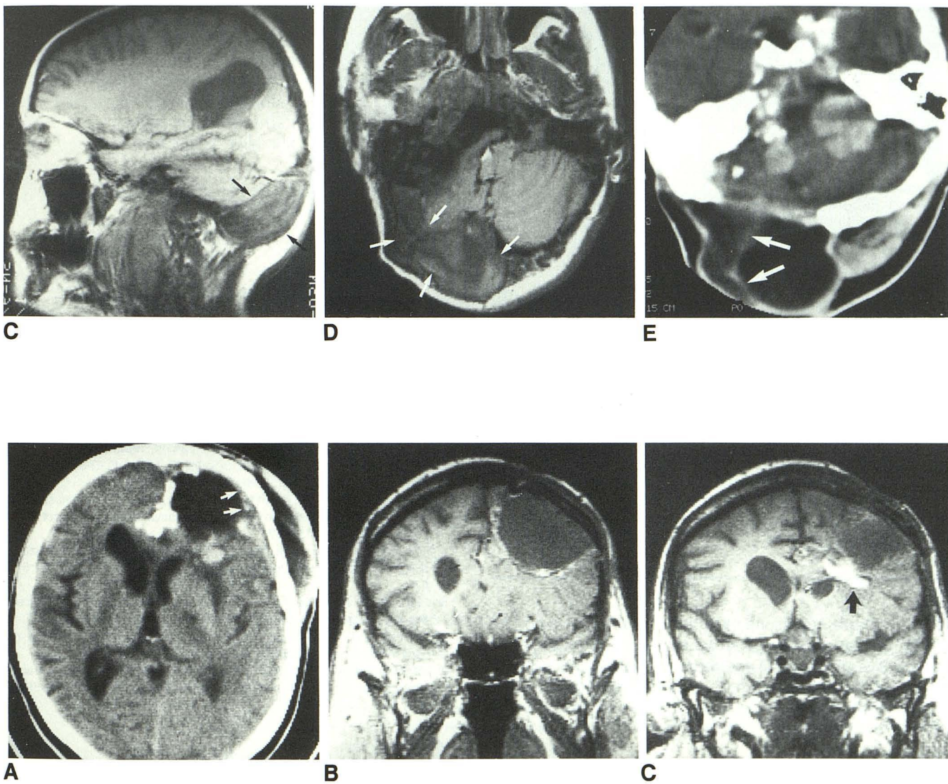
Fig. 7. —Cysts associated with recurrent tumor 6 months after left frontal craniotomy in patient with known oligodendroglioma. A, Follow-up CT study. Partially cystic, partially solid mass in left frontal region appears to be surrounded by thin rim of brain ( arrows ) and was interpreted as intraaxial and part of recurrent tumor. B, MR image (TR = 2000 msec, TE = 32 msec) reveals that cyst is extraaxial. C, Small nodule or recurrent tumor was found deep to cyst ( arrow ).
