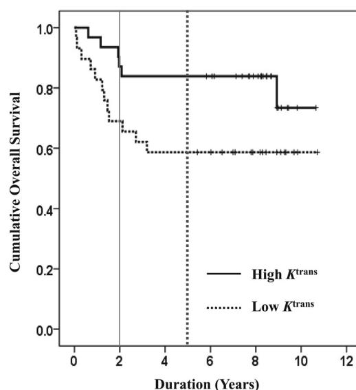
FIG 4. Kaplan-Meier plots for K^{\text{trans}} . Patients with higher pretreatment K^{\text{trans}} (solid curves) demonstrate longer OS compared with patients with lower K^{\text{trans}} (broken curves) at the 2-year (solid vertical line; P = .07 ), 5-year (dotted vertical line; P = .028 ), and long-term (median duration, >7 years; P = .06 ) follow-up periods.
