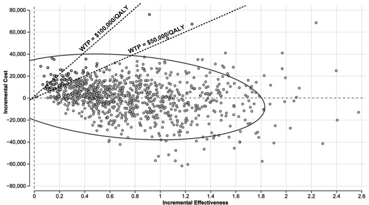
FIG 4. Probabilistic sensitivity analysis considering the collective variation of costs, utilities, imaging parameters, and radiation-induced toxicity risk with 100,000 iterations. The probabilistic sensitivity analysis showed that the new strategy is cost-effective in 91% of the 100,000 iterations, demonstrating its cost-effectiveness at WTP = $50,000/QALY.
